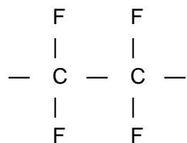
Teflon poly(tetrafluoroethene)
